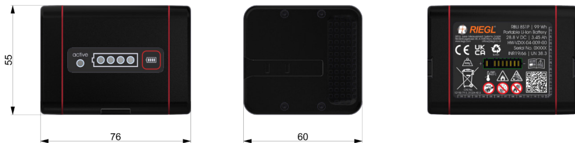
Fig. 1 Dimensional Drawing of the RIEGL RBLI 8S1P, all dimensions in mm
